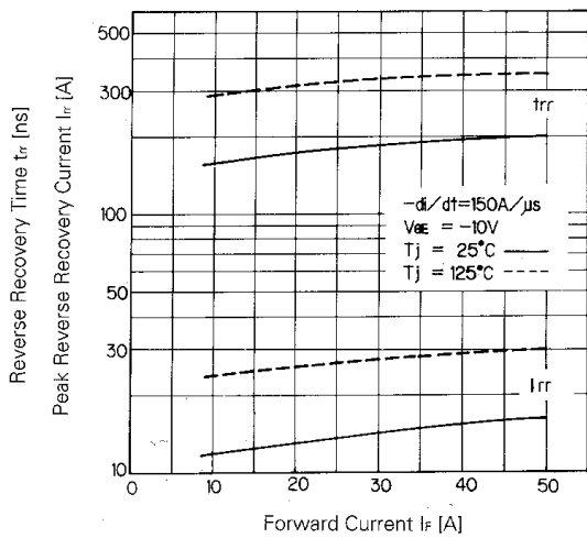
t_{rr}, I_{rr}-I_f
