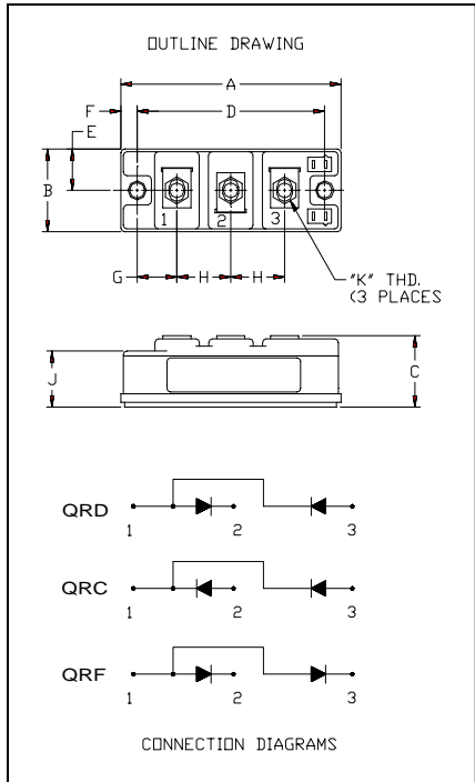
QR_0630T30 Fast Recovery Diode Module
